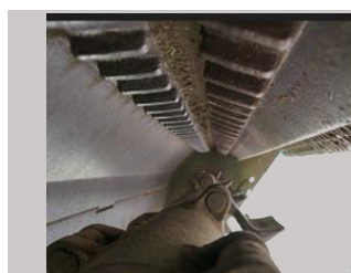
Replaceable drop forged re-cutter bars
